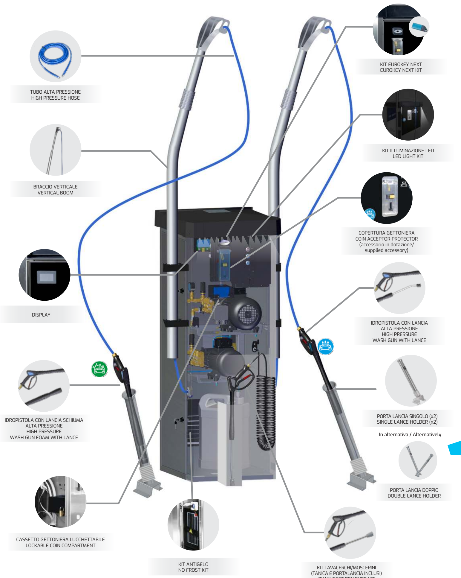
ACQUA IN ALTA PRESSIONE HIGH PRESSURE WATER
